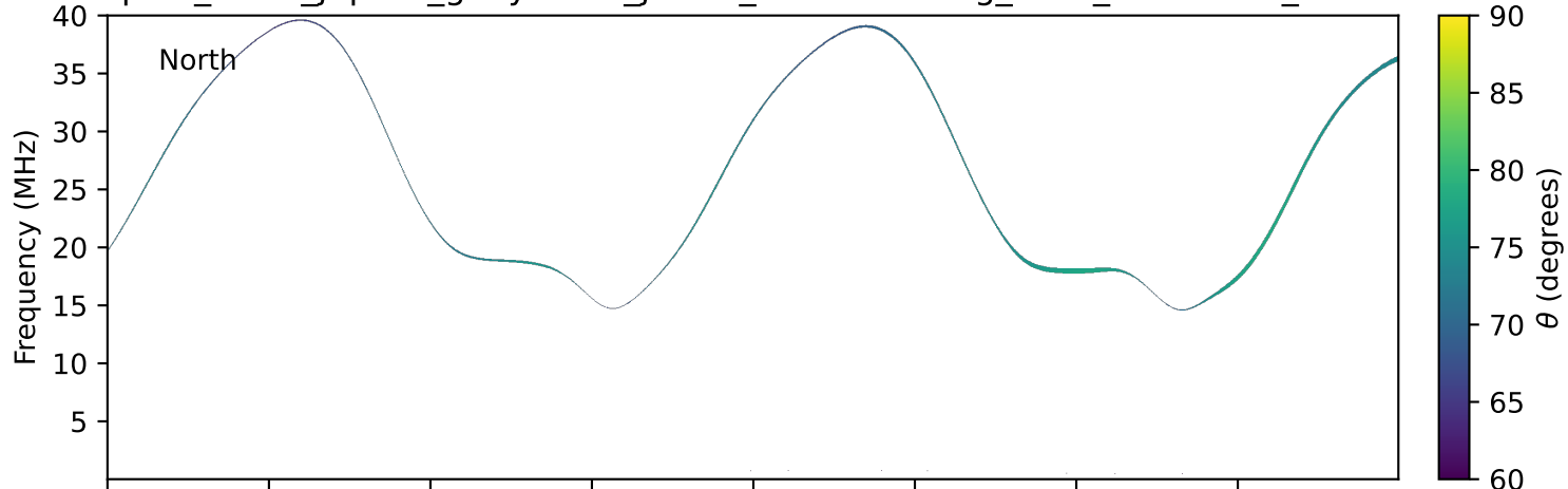
expres_earth_jupiter_ganymede_jrm33_lossc-wid1deg_3kev_20190304_v11.cdf
