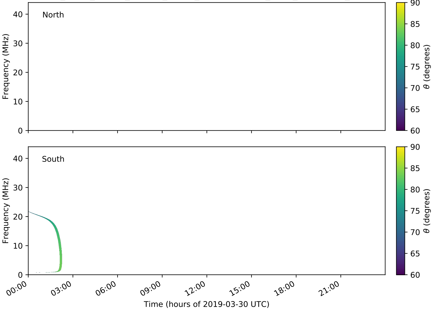
expres_earth_jupiter_europa_jrm09_lossc-wid1deg_3kev_20190330_v01.cdf
