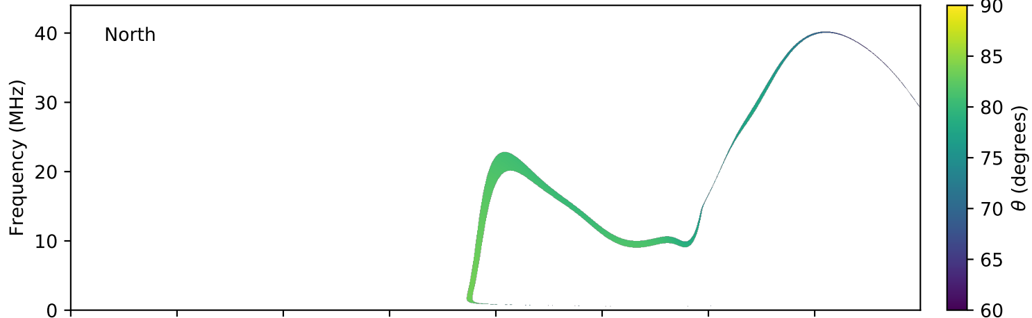
expres_earth_jupiter_europa_jrm09_lossc-wid1deg_3kev_20190328_v01.cdf
