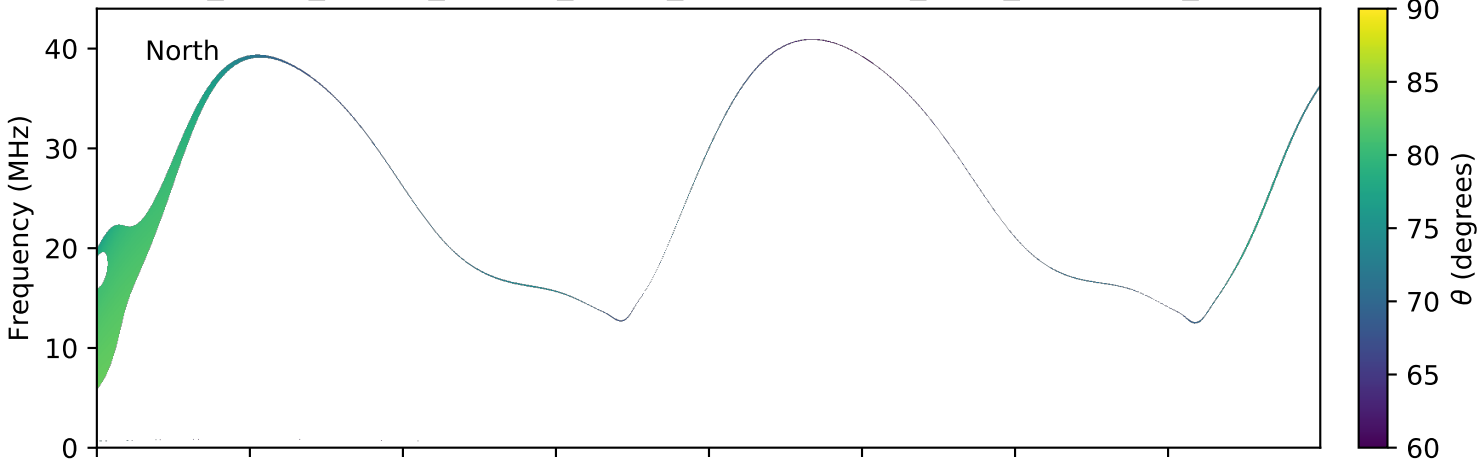
expres_earth_jupiter_europa_jrm09_lossc-wid1deg_3kev_20190318_v01.cdf
