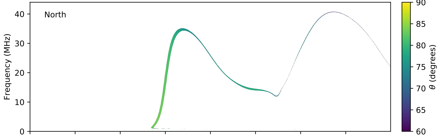
expres_earth_jupiter_europa_jrm09_lossc-wid1deg_3kev_20190314_v01.cdf
