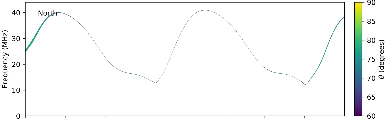
expres_earth_jupiter_europa_jrm09_lossc-wid1deg_3kev_20190311_v01.cdf
