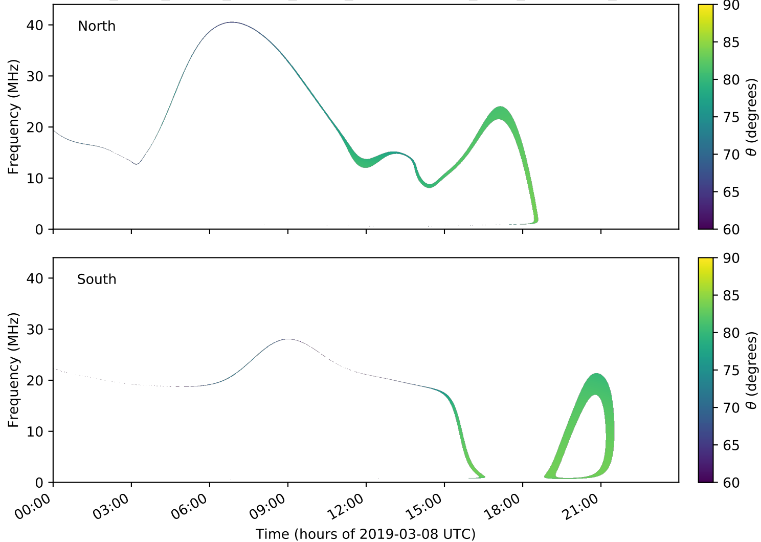
expres_earth_jupiter_europa_jrm09_lossc-wid1deg_3kev_20190308_v01.cdf
