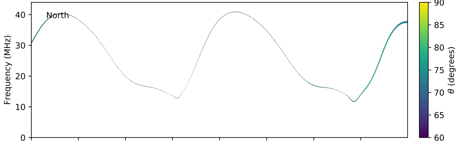
expres_earth_jupiter_europa_jrm09_lossc-wid1deg_3kev_20190304_v01.cdf
