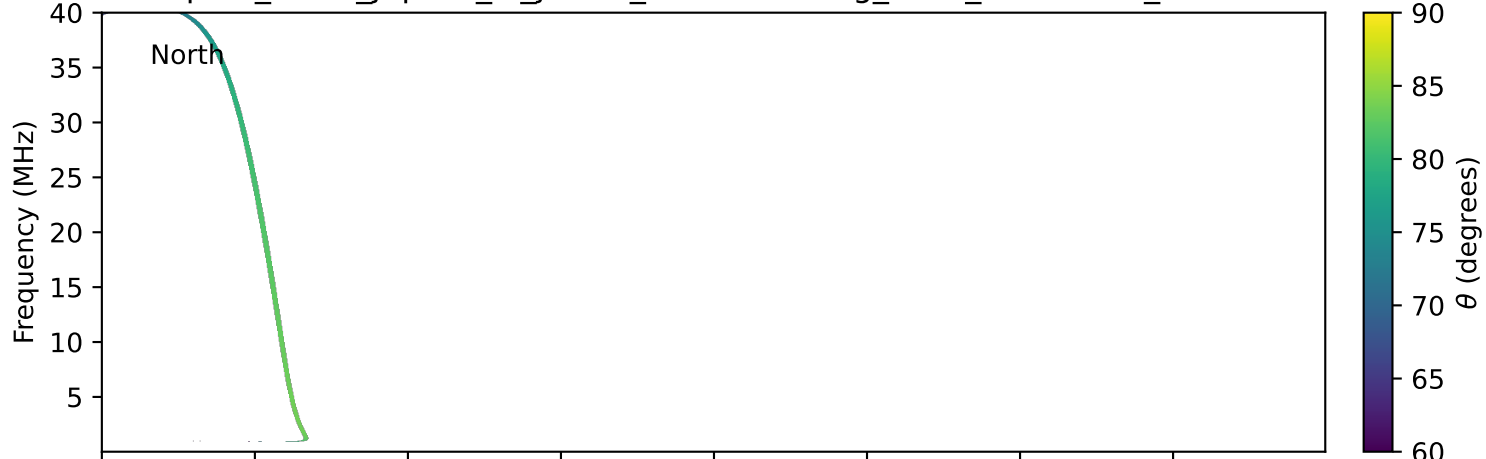
expres_earth_jupiter_io_jrm33_lossc-wid1deg_3kev_20190228_v11.cdf
