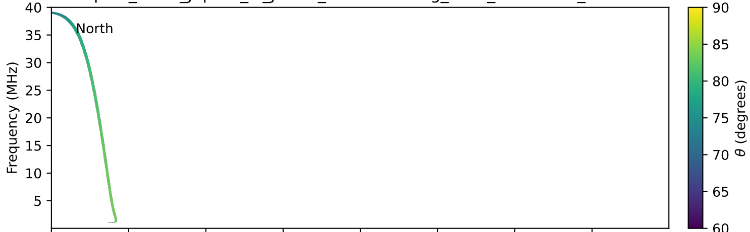
expres_earth_jupiter_io_jrm33_lossc-wid1deg_3kev_20190221_v11.cdf
