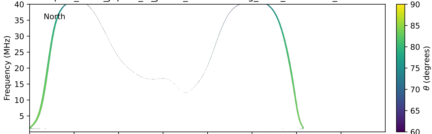
expres_earth_jupiter_io_jrm33_lossc-wid1deg_3kev_20190215_v11.cdf
