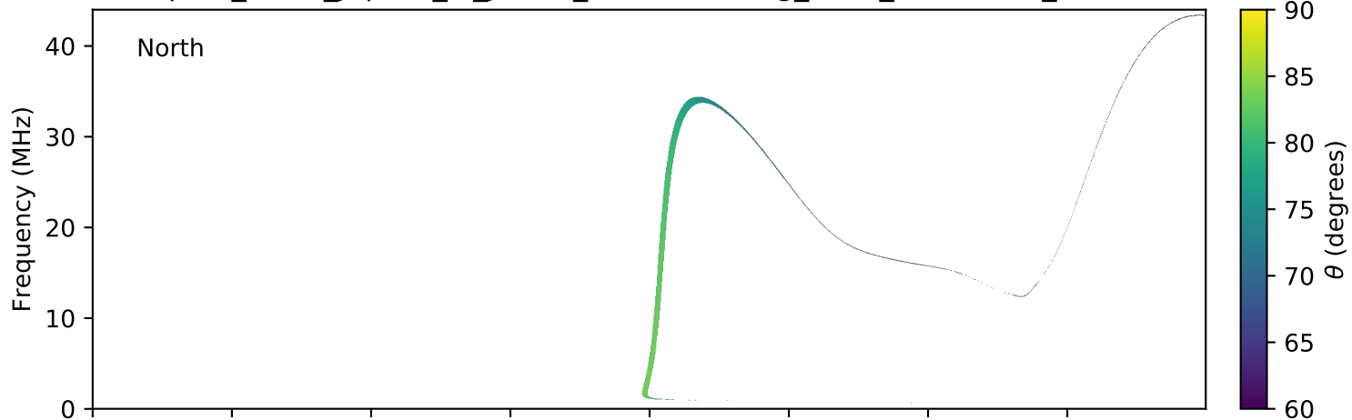
expres_earth_jupiter_io_jrm09_lossc-wid1deg_3kev_20190227_v01.cdf
