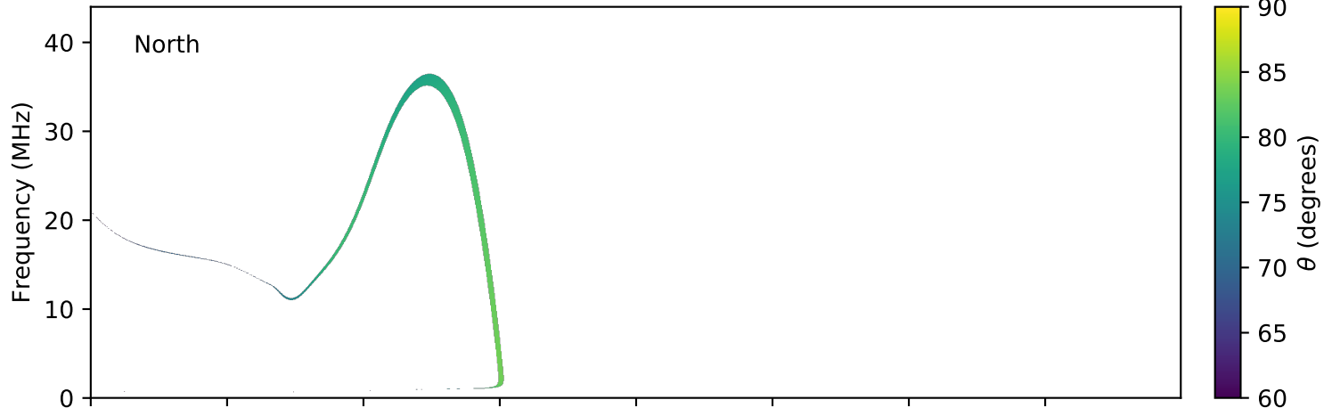
expres_earth_jupiter_io_jrm09_lossc-wid1deg_3kev_20190212_v01.cdf
