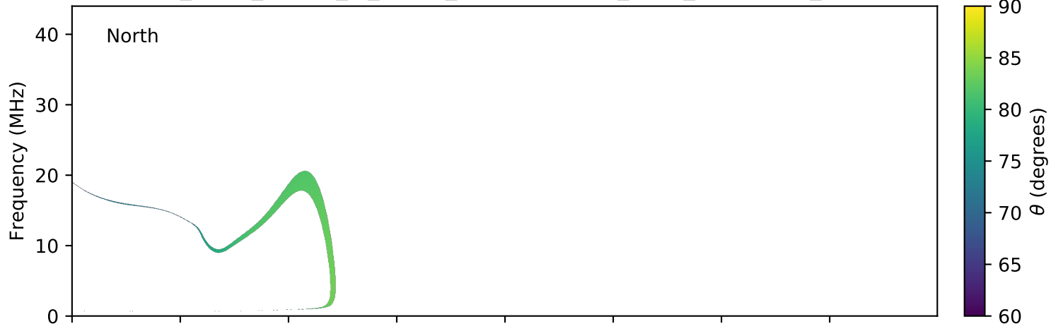
expres_earth_jupiter_io_jrm09_lossc-wid1deg_3kev_20190205_v01.cdf
