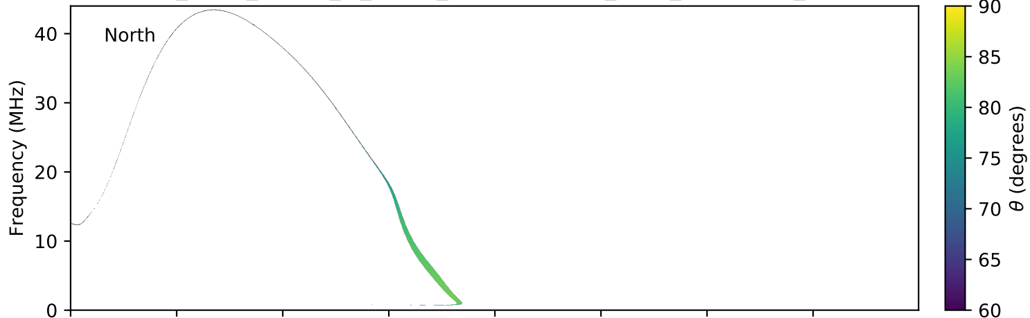
expres_earth_jupiter_io_jrm09_lossc-wid1deg_3kev_20190203_v01.cdf
