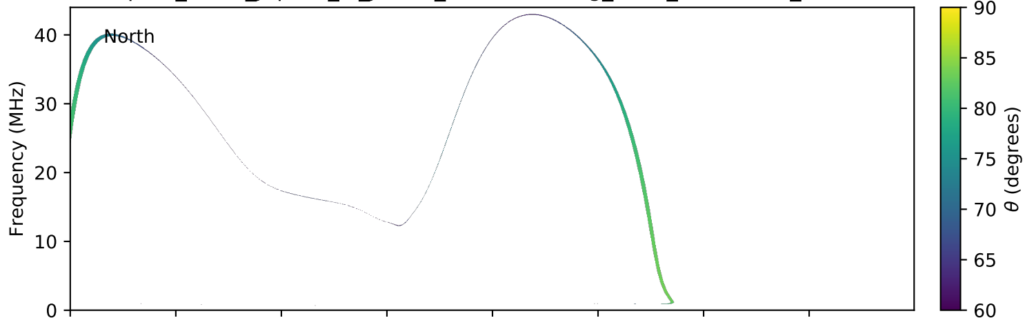
expres_earth_jupiter_io_jrm09_lossc-wid1deg_3kev_20190201_v01.cdf
