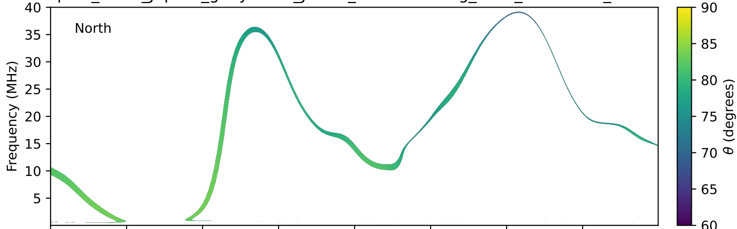
expres_earth_jupiter_ganymede_jrm33_lossc-wid1deg_3kev_20190209_v11.cdf
