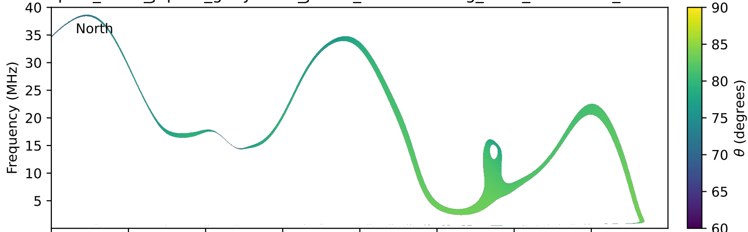
expres_earth_jupiter_ganymede_jrm33_lossc-wid1deg_3kev_20190204_v11.cdf
