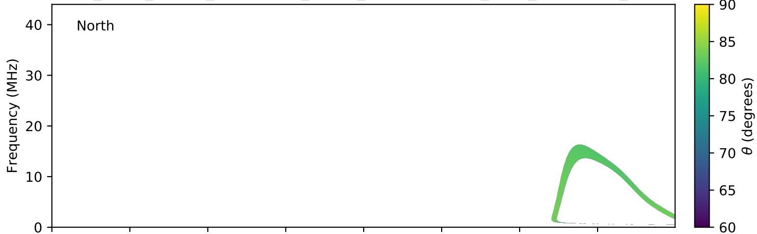
expres_earth_jupiter_ganymede_jrm09_lossc-wid1deg_3kev_20190223_v01.cdf
