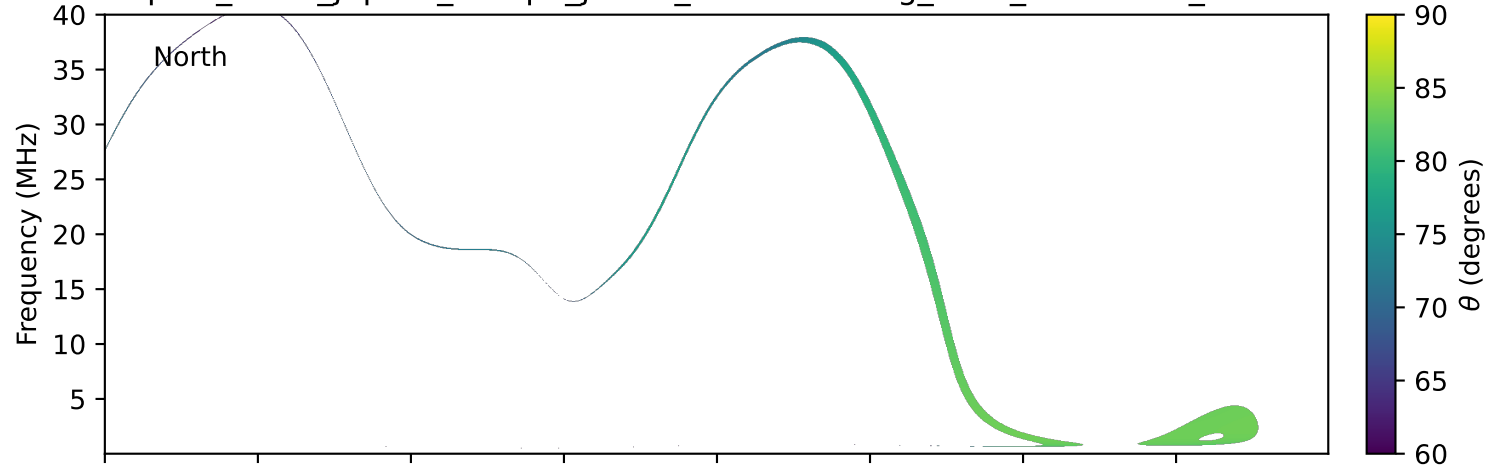
expres_earth_jupiter_europa_jrm33_lossc-wid1deg_3kev_20190225_v11.cdf
