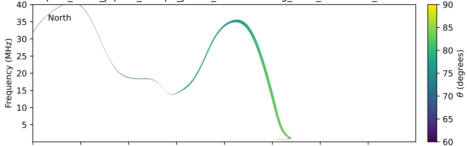
expres_earth_jupiter_europa_jrm33_lossc-wid1deg_3kev_20190218_v11.cdf
