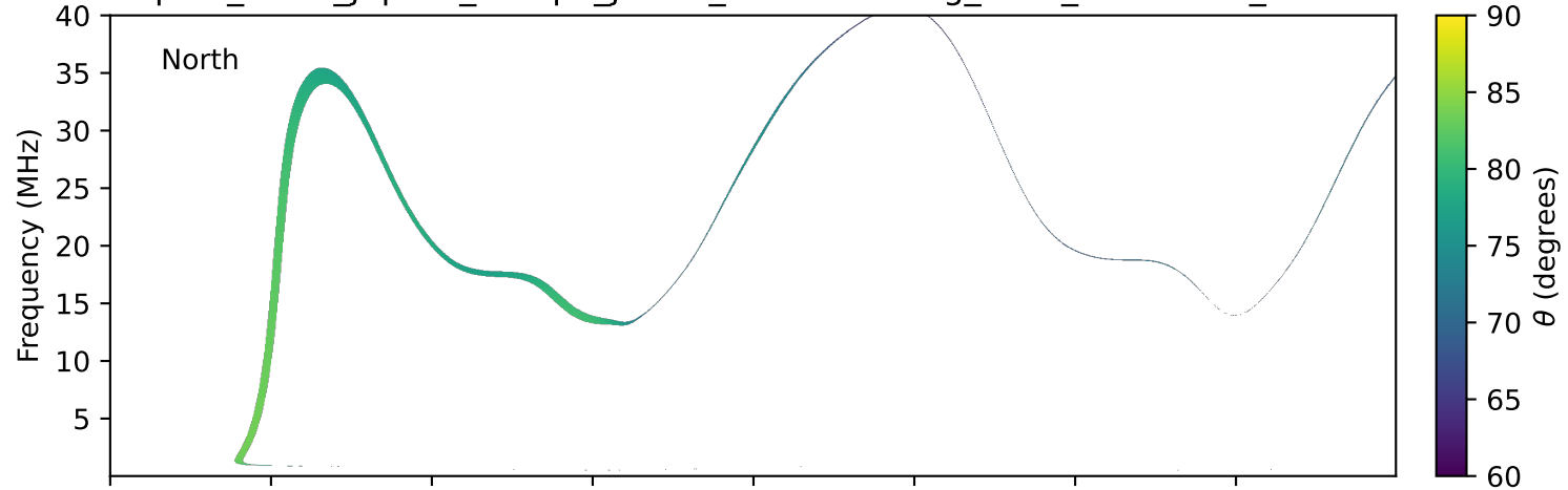
expres_earth_jupiter_europa_jrm33_lossc-wid1deg_3kev_20190210_v11.cdf
