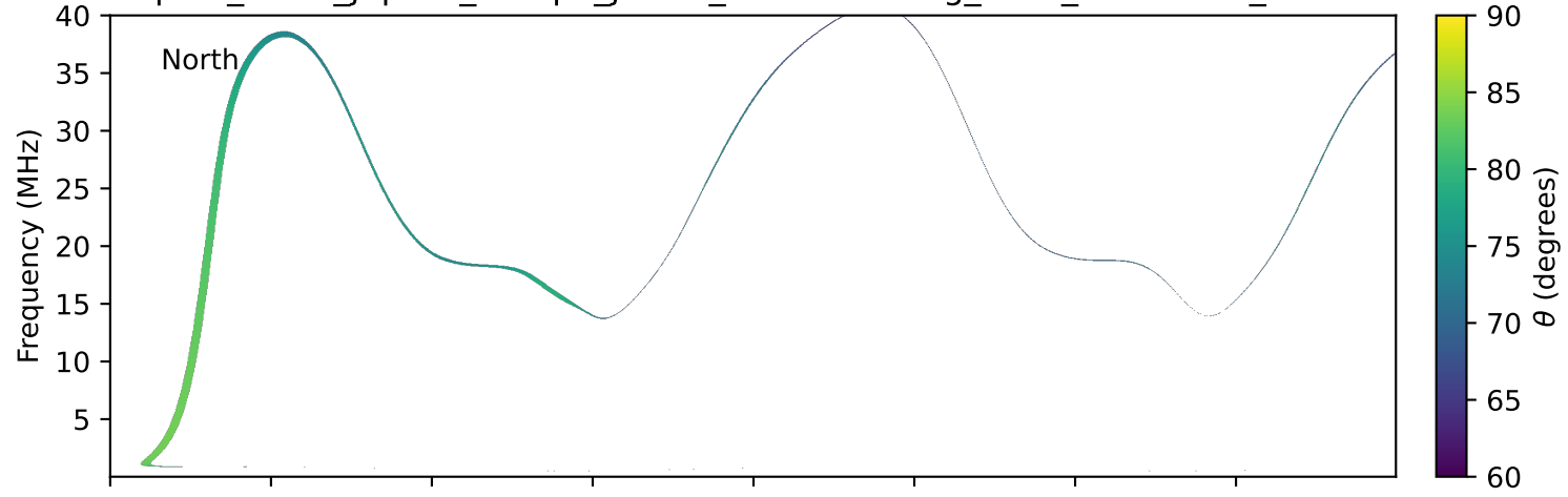
expres_earth_jupiter_europa_jrm33_lossc-wid1deg_3kev_20190203_v11.cdf
