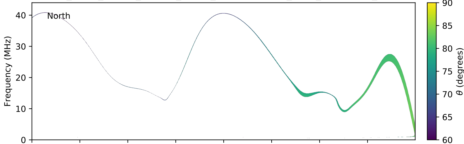
expres_earth_jupiter_europa_jrm09_lossc-wid1deg_3kev_20190218_v01.cdf
