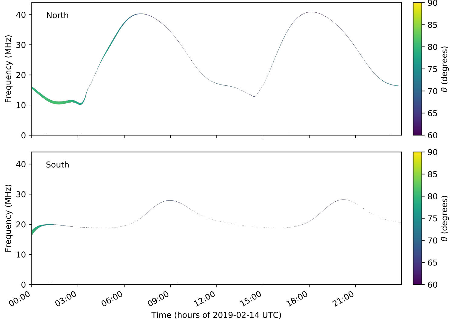
expres_earth_jupiter_europa_jrm09_lossc-wid1deg_3kev_20190214_v01.cdf
