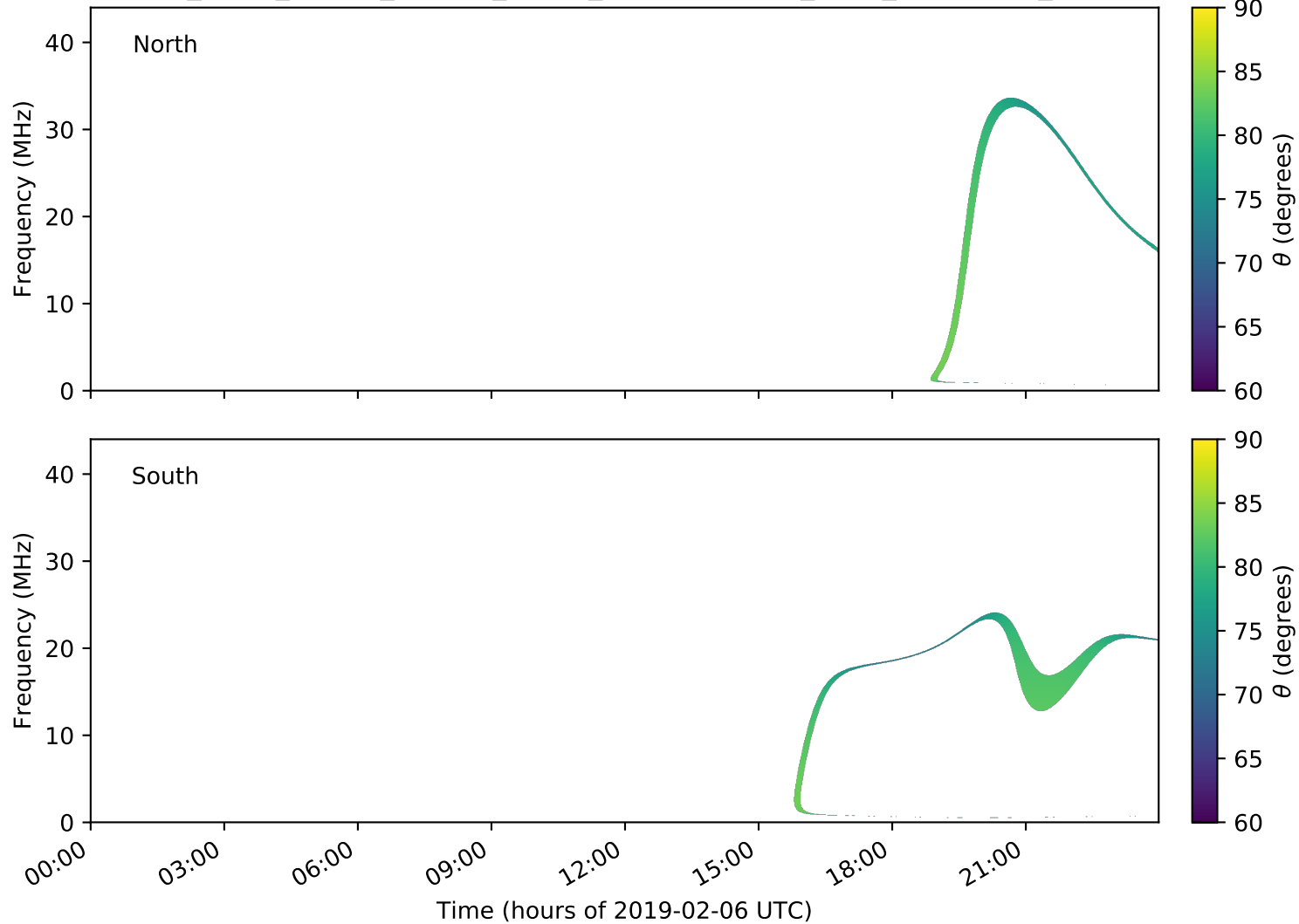
expres_earth_jupiter_europa_jrm09_lossc-wid1deg_3kev_20190206_v01.cdf
