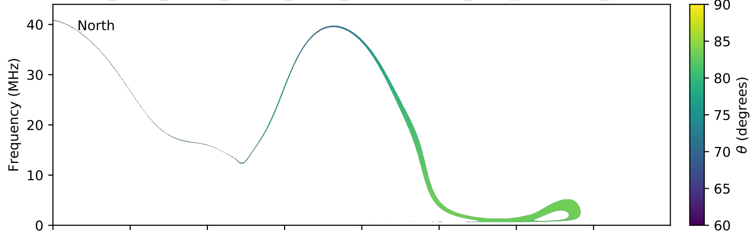
expres_earth_jupiter_europa_jrm09_lossc-wid1deg_3kev_20190204_v01.cdf
