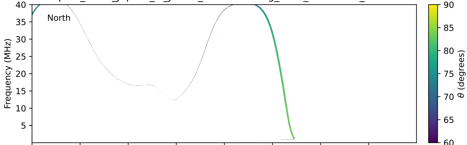
expres_earth_jupiter_io_jrm33_lossc-wid1deg_3kev_20181220_v11.cdf
