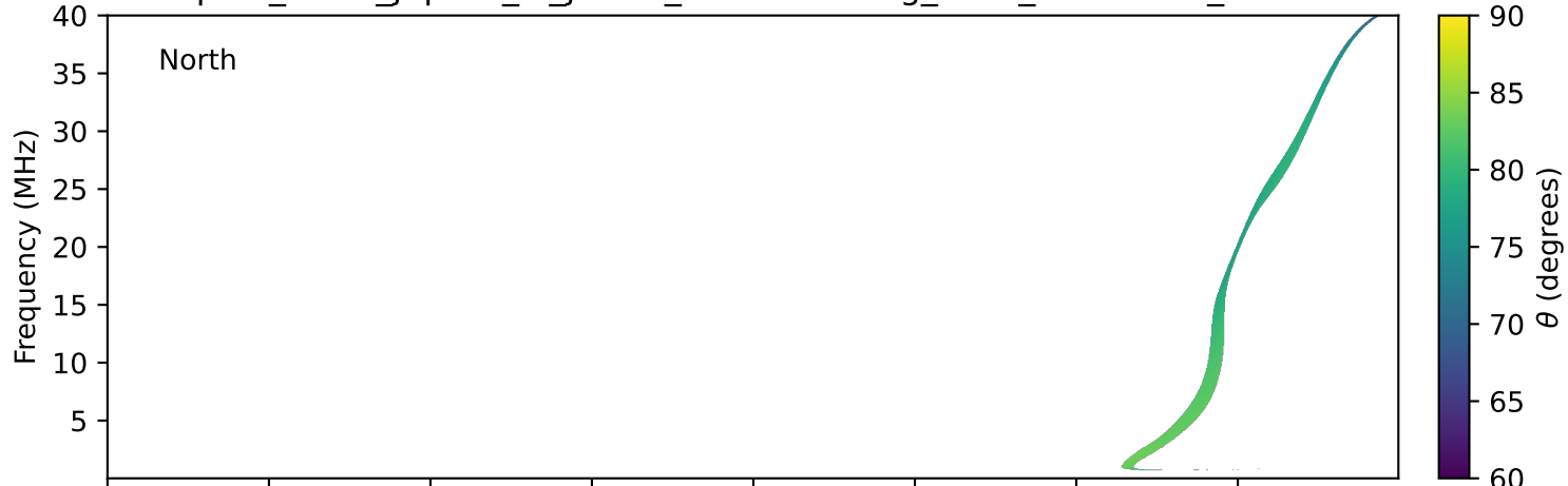
expres_earth_jupiter_io_jrm33_lossc-wid1deg_3kev_20181212_v11.cdf
