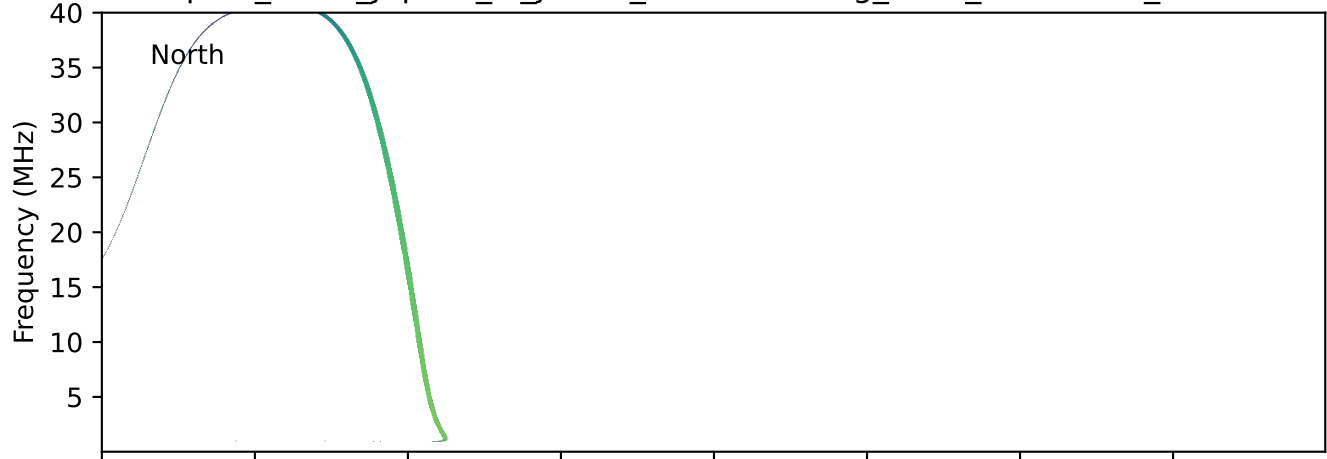
expres_earth_jupiter_io_jrm33_lossc-wid1deg_3kev_20181208_v11.cdf
