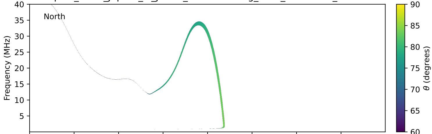
expres_earth_jupiter_io_jrm33_lossc-wid1deg_3kev_20181206_v11.cdf
