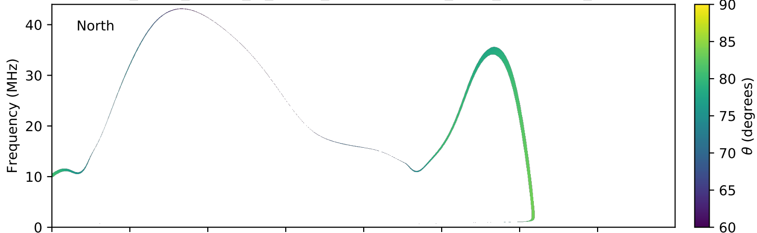
expres_earth_jupiter_io_jrm09_lossc-wid1deg_3kev_20181231_v01.cdf
