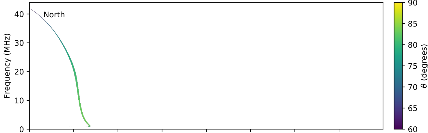
expres_earth_jupiter_io_jrm09_lossc-wid1deg_3kev_20181228_v01.cdf
