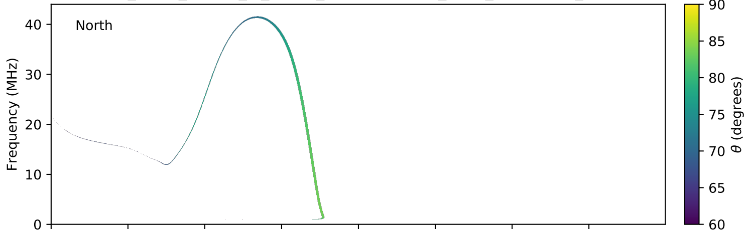
expres_earth_jupiter_io_jrm09_lossc-wid1deg_3kev_20181226_v01.cdf
