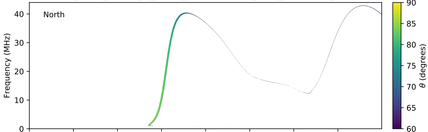
expres_earth_jupiter_io_jrm09_lossc-wid1deg_3kev_20181220_v01.cdf
