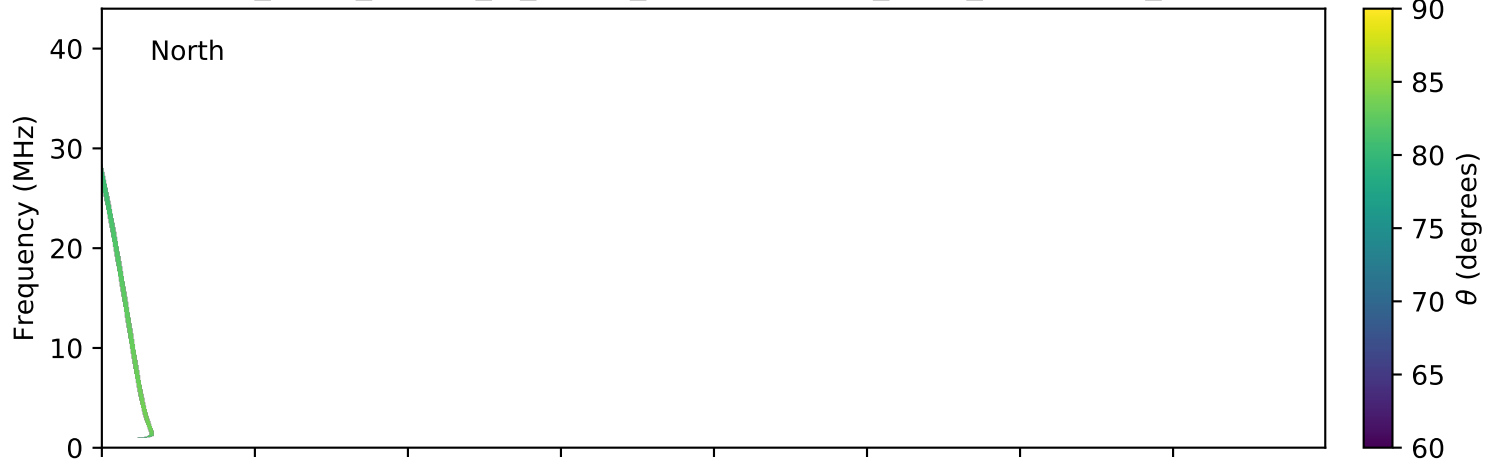
expres_earth_jupiter_io_jrm09_lossc-wid1deg_3kev_20181214_v01.cdf
