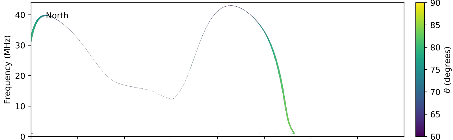
expres_earth_jupiter_io_jrm09_lossc-wid1deg_3kev_20181208_v01.cdf
