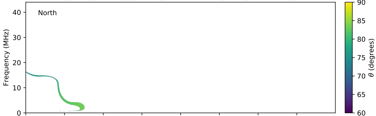
expres_earth_jupiter_io_jrm09_lossc-wid1deg_3kev_20181205_v01.cdf
