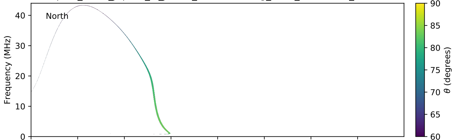
expres_earth_jupiter_io_jrm09_lossc-wid1deg_3kev_20181203_v01.cdf
