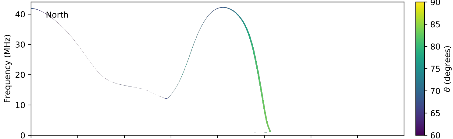
expres_earth_jupiter_io_jrm09_lossc-wid1deg_3kev_20181201_v01.cdf
