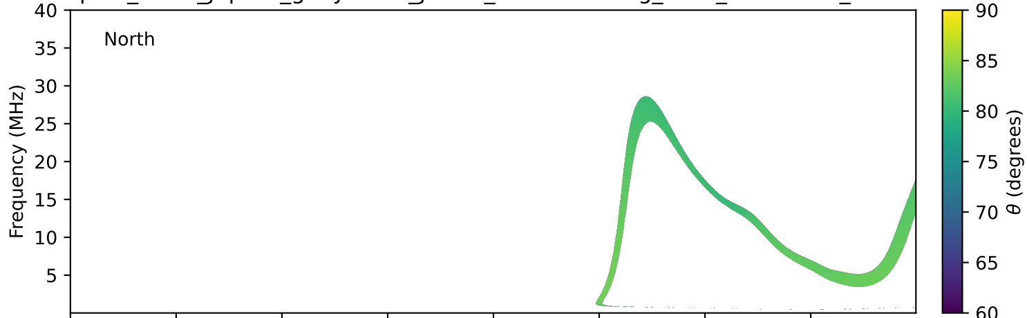
expres_earth_jupiter_ganymede_jrm33_lossc-wid1deg_3kev_20181202_v11.cdf
