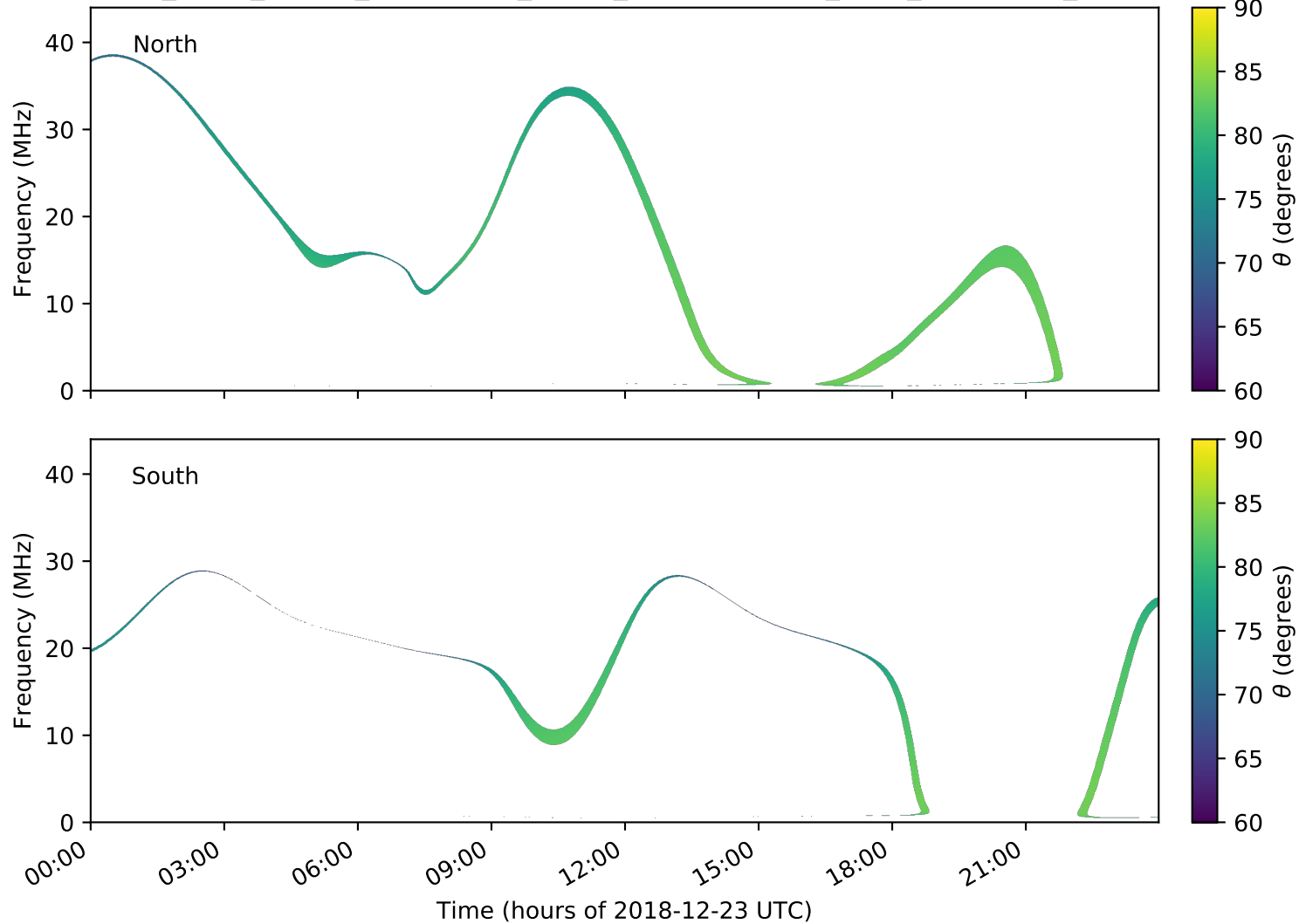
expres_earth_jupiter_ganymede_jrm09_lossc-wid1deg_3kev_20181223_v01.cdf
