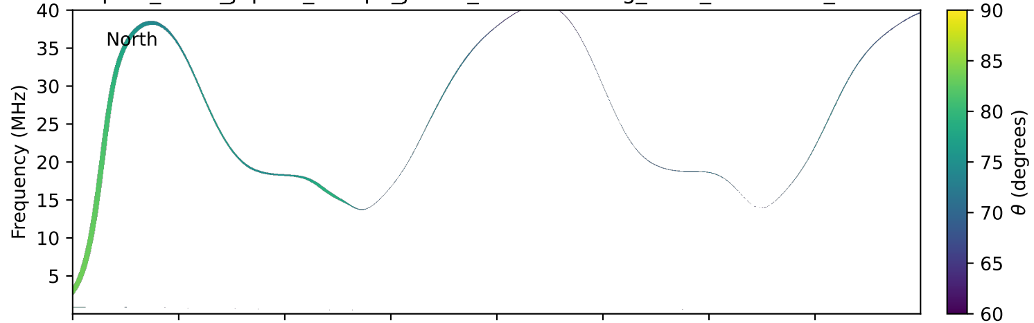
expres_earth_jupiter_europa_jrm33_lossc-wid1deg_3kev_20181203_v11.cdf
