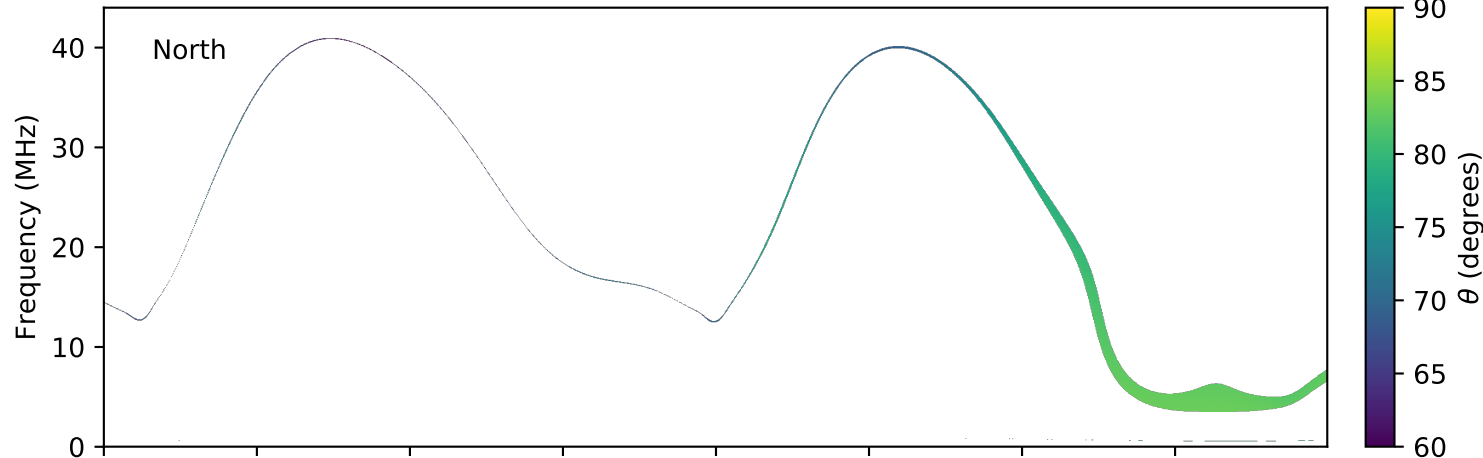
expres_earth_jupiter_europa_jrm09_lossc-wid1deg_3kev_20181205_v01.cdf
