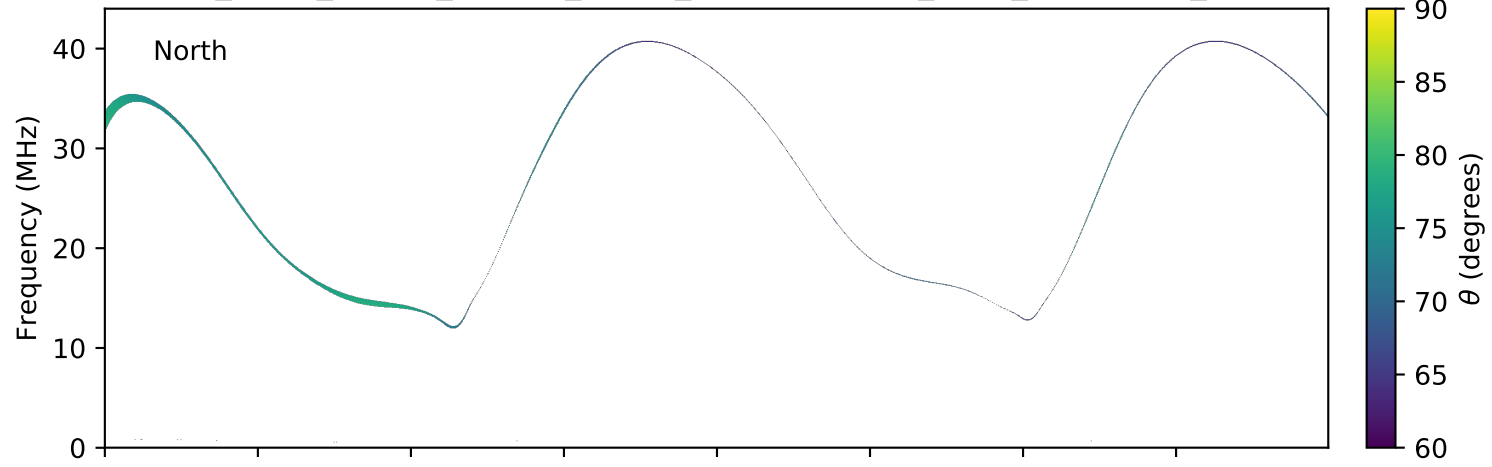
expres_earth_jupiter_europa_jrm09_lossc-wid1deg_3kev_20181201_v01.cdf
