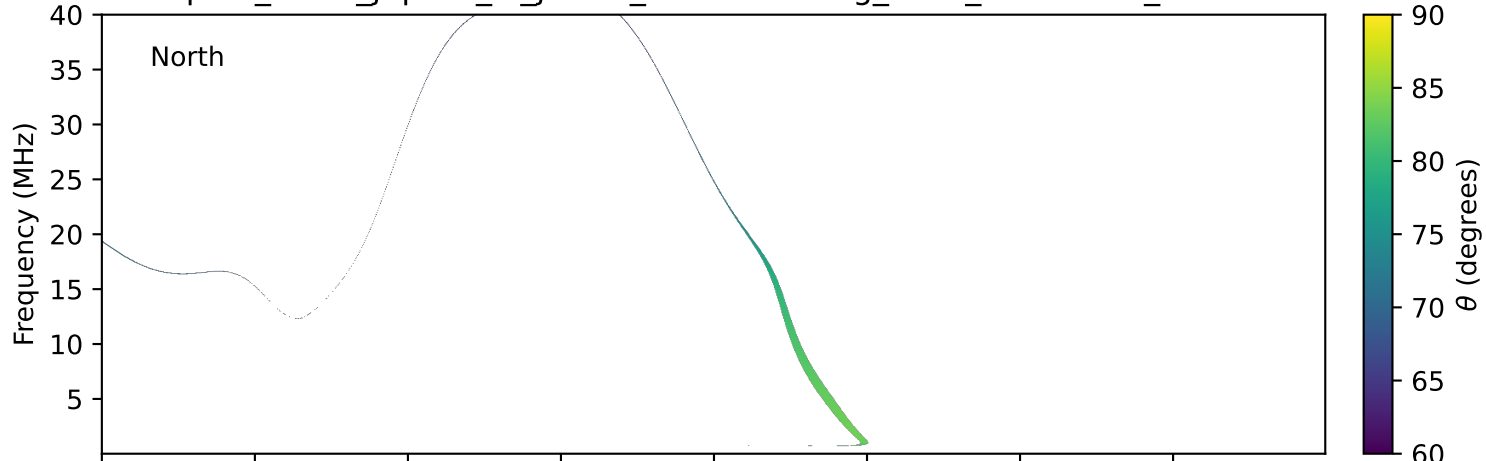
expres_earth_jupiter_io_jrm33_lossc-wid1deg_3kev_20181127_v11.cdf
