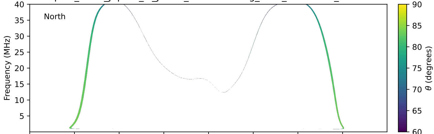
expres_earth_jupiter_io_jrm33_lossc-wid1deg_3kev_20181125_v11.cdf
