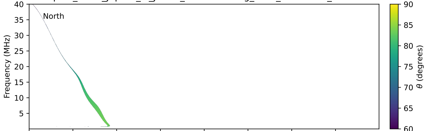
expres_earth_jupiter_io_jrm33_lossc-wid1deg_3kev_20181115_v11.cdf
