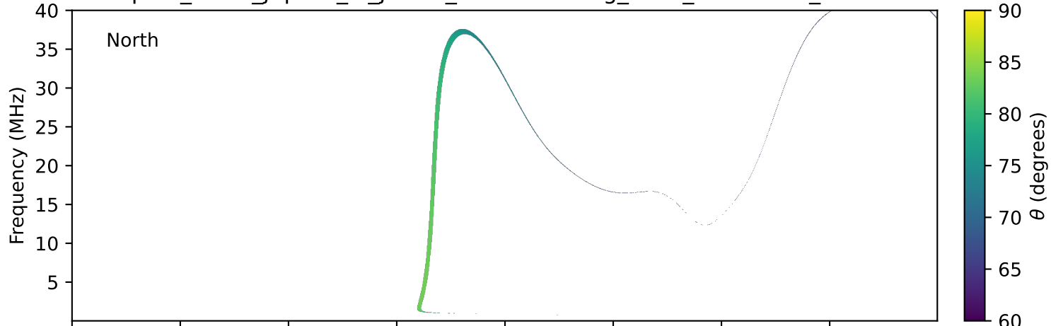
expres_earth_jupiter_io_jrm33_lossc-wid1deg_3kev_20181107_v11.cdf
