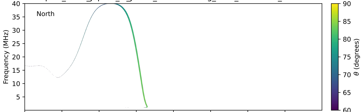
expres_earth_jupiter_io_jrm33_lossc-wid1deg_3kev_20181106_v11.cdf
